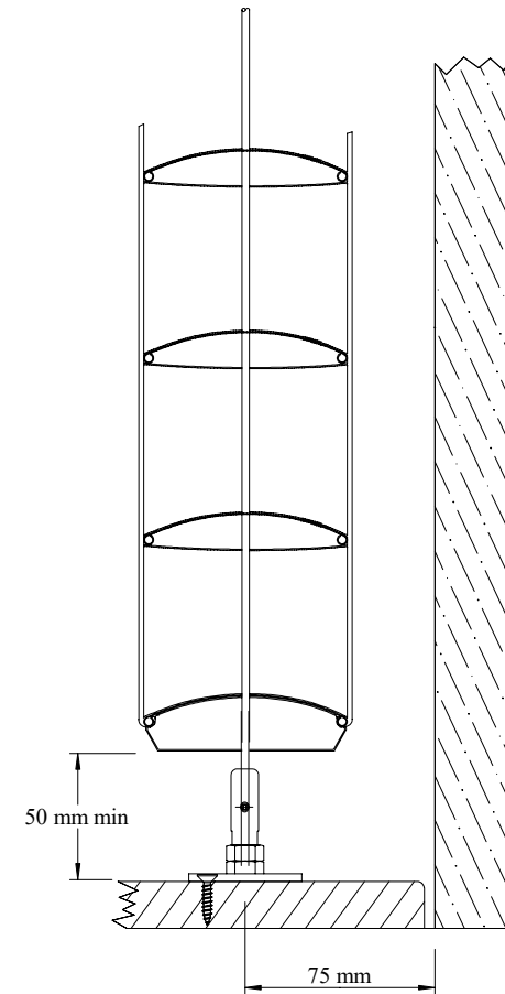
Typical Fixing
