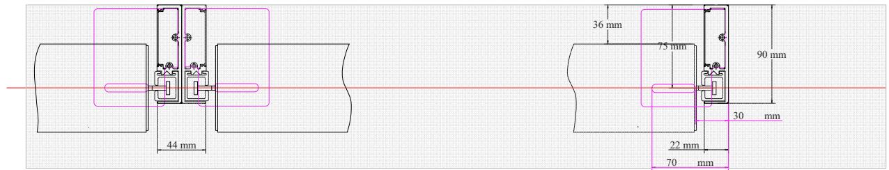
Typical Fixing
